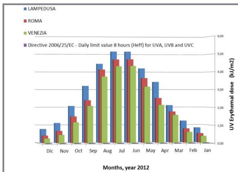
Figure 1. Comparison of the average daily erythemal dose among three Italian regions during the year 2012
