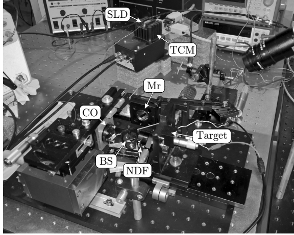
Fig. 4. Picture of the developed measuring system. In the figure it is possible to see the collimator CO, the beam-splitter BS, the neutral density filter NDF, the Target, the mirror Mr, the SLD and the temperature-controlled mount TCM.
