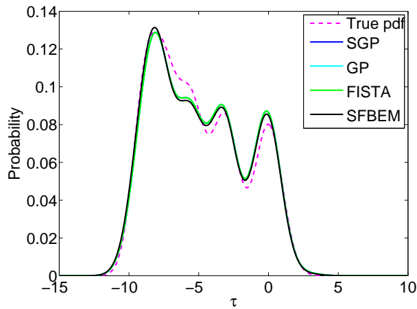
Figure 5: Density estimation results.
