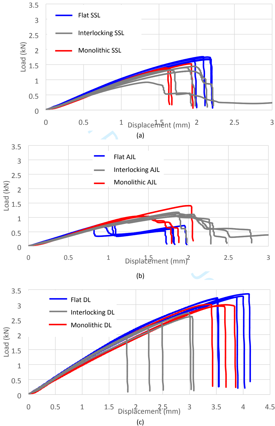
Figure 8 – Experimental Load Displacement curves for SSLs (a) AJLs (b) and DLJs (c). Blue curves represent the flat configuration, gray curves the interlocking joints and red curves the monolithic ones.
