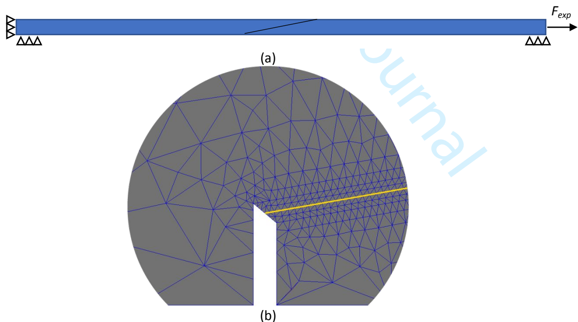
16 Figure 7 –FE model loading scheme, scale 1:1 (a), mesh details with the midline of the adhesive in yellow (b)
