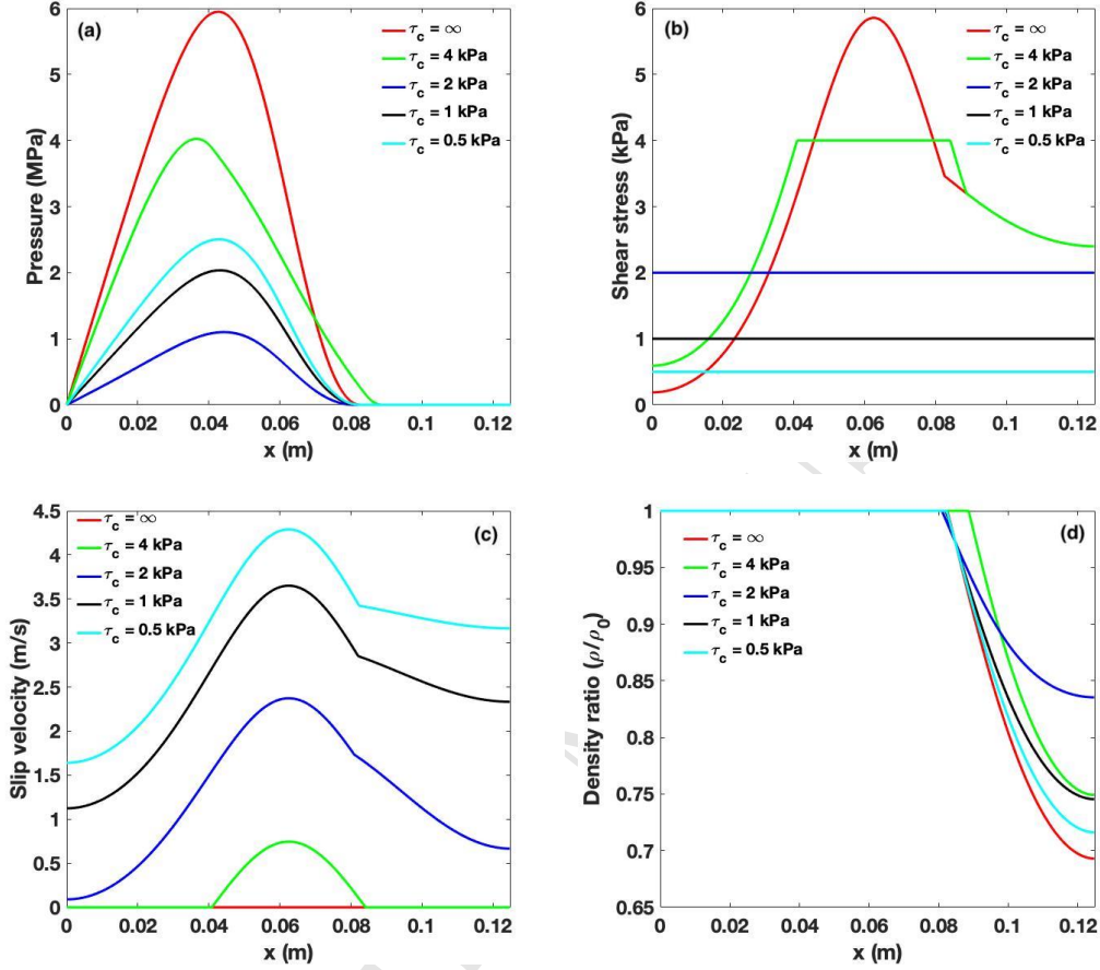
Figure 6: Pressure (a), shear stress (b), slip velocity (c) and density ratio (d) for the cosine profile for several values of uniform \tau_c .
