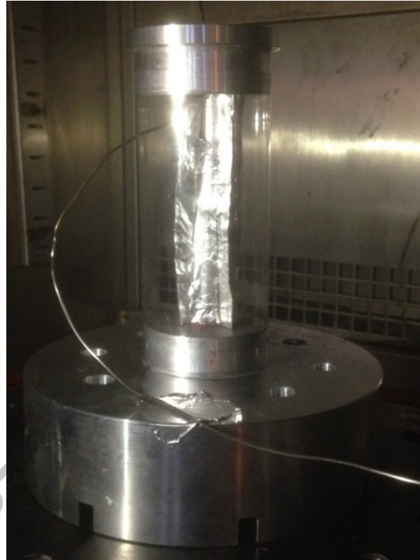
Figure 9 – Set-up for axial forcing load tests with thermic gradient
