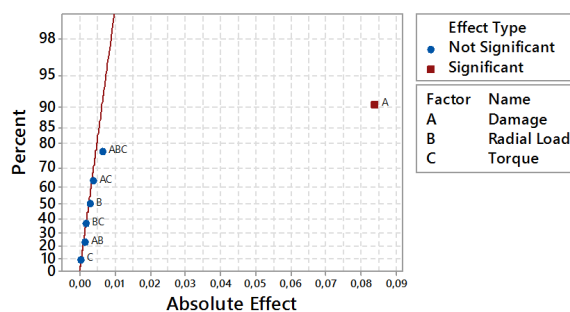
Fig. 12. Test set 1 (single point defect on outer race): Half normal plot of the scalar current fault indicator.
