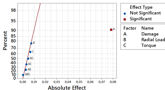
Fig. 14. Test set 2 (brinnelling defect): Half normal plot of the scalar current fault indicator.
