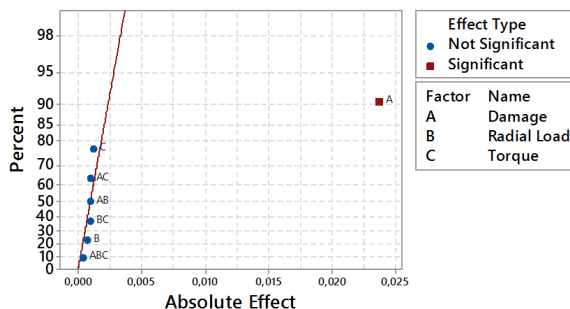
Fig. 13. Test set 2 (brinnelling defect): Half normal plot of the scalar vibration fault indicator.
