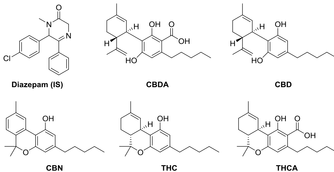
Figure 1. Molecular structure of Diazepam (IS), CBD-A, CBD, CBN, THC and THC-A.
