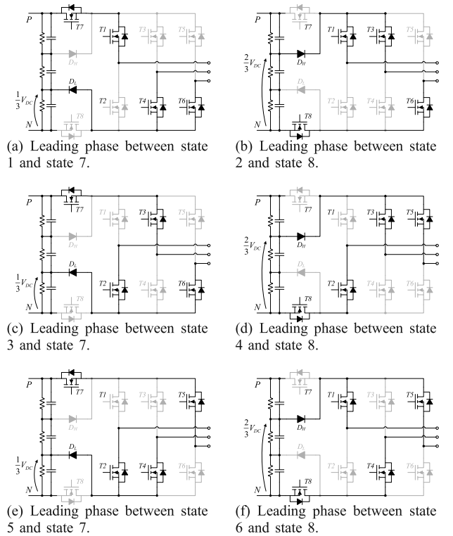
Figure 10. Configurations of the H8 inverter during transitions from active to inactive states. Devices are depicted in black if they are on, in gray if they are off. Current conduction through anti-parallel diodes are neglected for simplicity.
