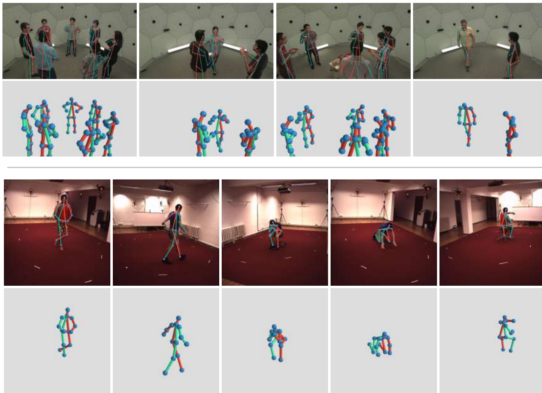
Fig. 11. Qualitative results of our LoCO approach. 1 st and 2 nd rows: result of LoCO on the CMU Panoptic dataset; 3 rd and 4 th rows: result of LoCO on the Human3.6m dataset. The Figure is taken from “Compressed Volumetric Heatmaps for Multi-Person 3D Pose Estimation” [15].
