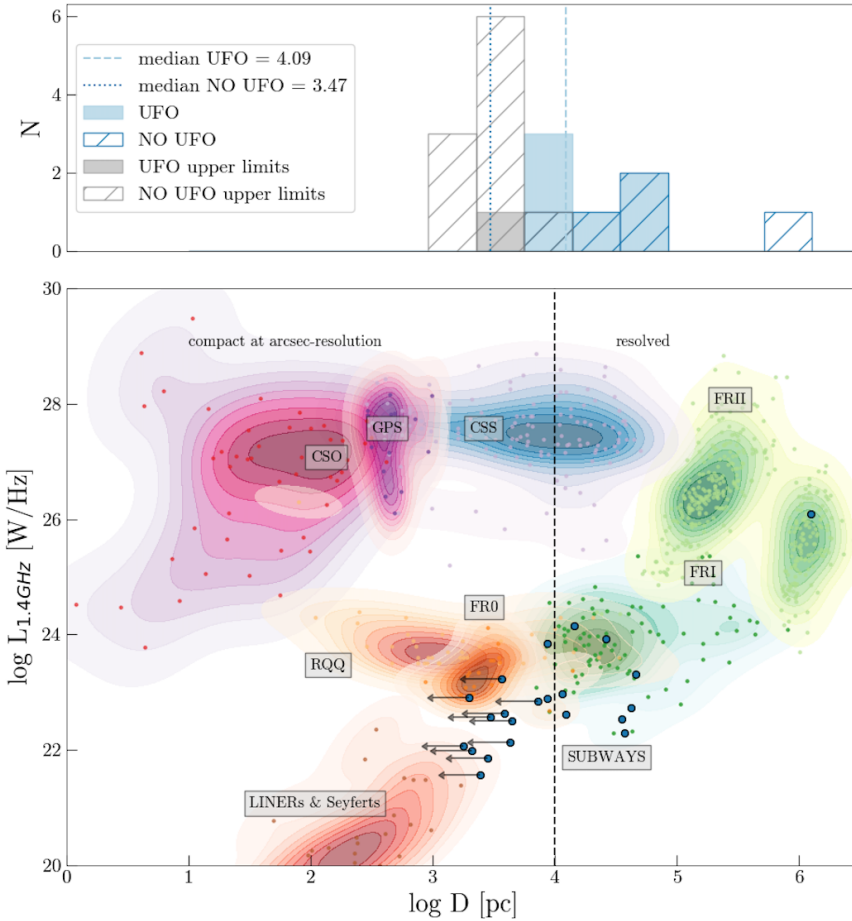
Fig. 5. Radio power at 1.4 GHz versus linear size plot (P-D diagram) for different types of RL and RQ AGNs, adapted from Baldi (2023). Points show individual objects and coloured contours represent a smoothed estimator of source density. The different categories of source shown are: CSO (compact symmetric objects), GPS (GHz-peaked spectrum sources), CSS (compact steep spectrum sources), FRI, FRII, RQ quasars, Seyferts and LINERS, and FR0s. The vertical dashed line roughly marks the separation between resolved and unresolved compact sources based on arcsecond angular resolution. The blue dots represent how SUBWAYS AGNs overlap to LINERS & Seyferts, FRI, FR0s and RQQ. PG1425+267 is a strong outlier, falling on the FRII region. Such variety is consistent with the sample being selected based on its X-ray properties. In the upper panel we show the linear size distribution of the sample, with the UFO-subsample (filled histogram) separated from the non-UFO one (barred histogram). The median physical size measured for the UFO subsample is higher ( 12.35 \pm 5 kpc) with respect to the non-UFO one ( 2.96 \pm 1 kpc), potentially supporting multi-phase outflow models (e.g. Crenshaw et al. 2003). Medians are computed taking into account the upper limits through KM survival analysis. Catalogue references: LINERS & Seyferts (Baldi et al. 2018), FR0 (Baldi et al. 2019; Cheng & An 2018); RQQ (Jarvis et al. 2021); GPS (Liu et al. 2007); CSS (Kunert-Bajraszewska et al. 2010); CSO (An & Baan 2012); FRI (Dabhade et al. 2020; Jimenez-Gallardo et al. 2019); FRII (Lao et al. 2024; Fanti et al. 1987).
