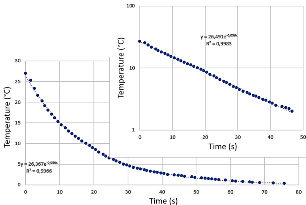
Figure 3. The exponential temperature versus time (the temperature is in log scale in the inset) obtained by a student in a measurement of time response for the digital thermometer (in air).
