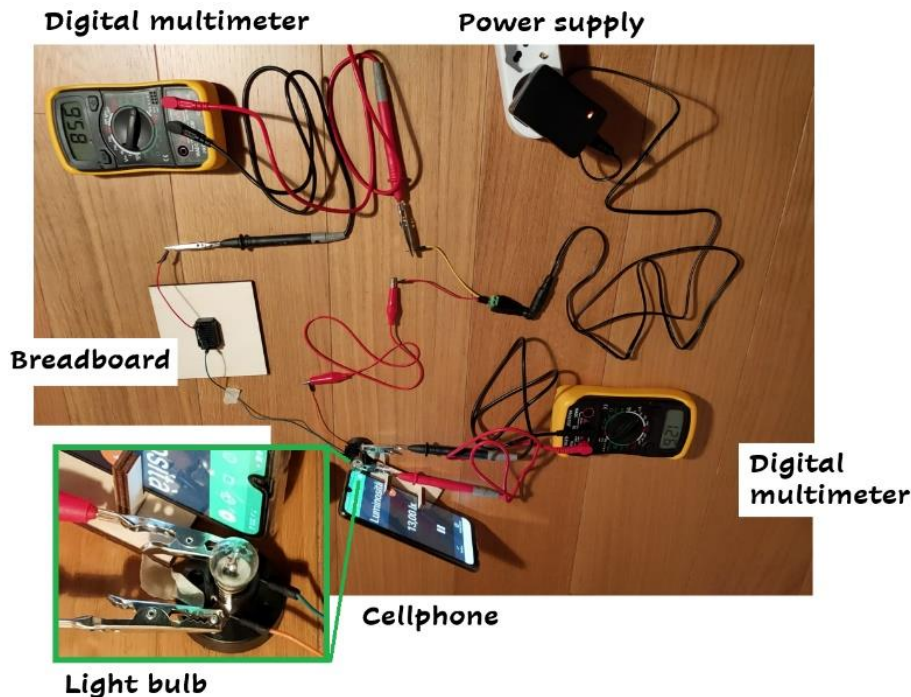
Figure 6. Two digital multimeters are involved, one to measure the potential difference V across the incandescent bulb and the other used as ammeter to measure the current I through the bulb. A resistor (chosen from those available in the kit) is placed on a breadboard in series with the lamp in order to obtain different voltage values from those supplied by the power supply (with nominal voltages of 3/4/5/6/7,5/9/12 V).
