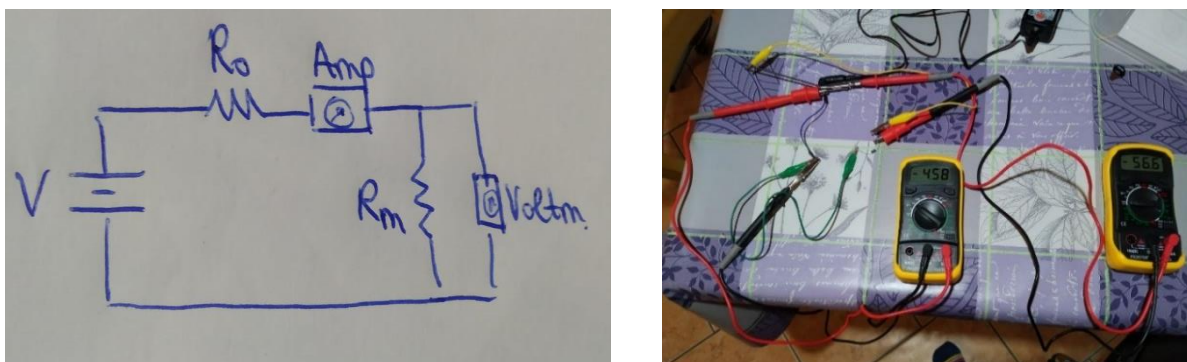
Figure 5. Experimental apparatus used by a student to measure the resistance of a graphite tab.
