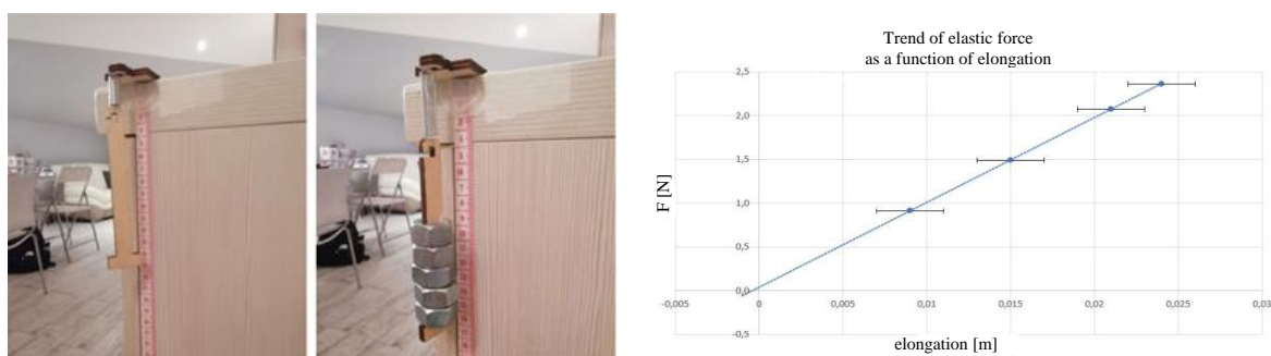
Figure 1. (Left) The experimental apparatus for the Hooke's law and (Right) an example of experimental data obtained and analyzed by a student at home.
