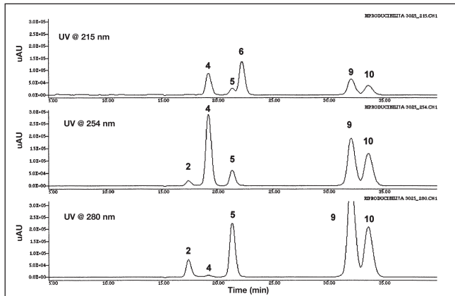
Figure 5. Chromatograms of standard solution. For peak identification, see Table I. Other conditions: flow, 0.6 mL/min; mobile phase, 0.01 N phosphoric acid (86%)–ACN (14%); and temperature, 22°C.
