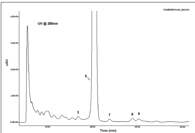
Figure 7. Chromatogram of authentic TBV sample showing the unknown peaks 3, 7, and 8.
