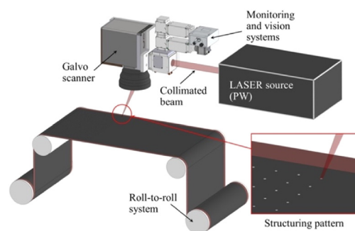
Fig. 12. Schematic of a laser-based electrode structuring process in a roll-to-roll system with the resulting micro-structured pattern (holes) on the moving electrode surface.
