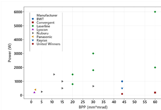
Fig. 7. Distribution of the industrial diode laser sources operating at blue wavelength as a function of beam parameter product (BPP) and power. All data were acquired by 26 May 2025.
