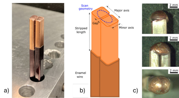
Fig. 18. a) Hairpin couples prepared for welding showing the stripped region and the cut flat surface. b) Schematic description of the weld scan trajectory in laser welding. c) The morphology of the weld bead.
